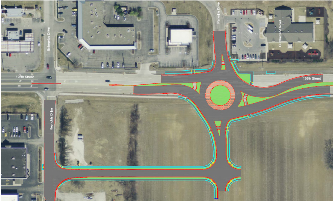
Rendering of new roundabout at 126th Street and Parkside Drive
