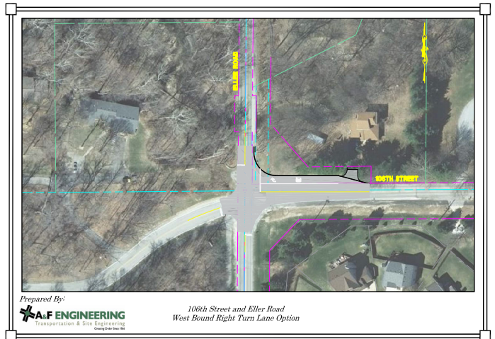
Rendering of the proposed intersection.
